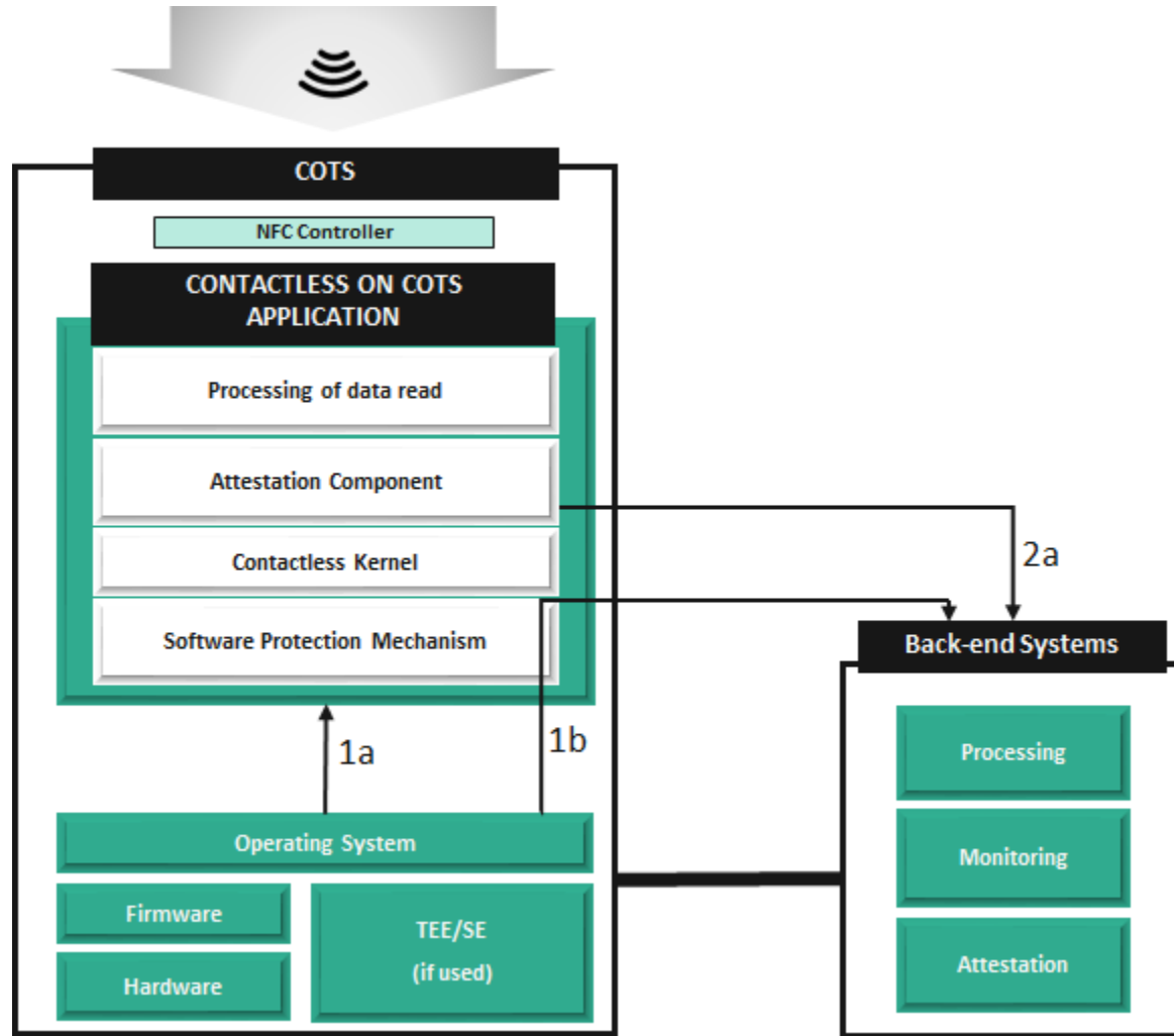
Figure 5: Attestation Flows
